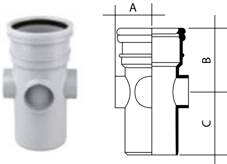
Unequal Branch (3 way bossed pipe. All bosses molded solid)
