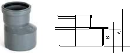
Eccentric Reducer (Sockets / Spigot) Short
