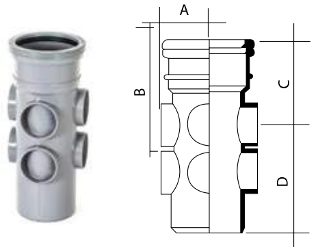
Unequal Branch (6 way bossed pipe. All bosses molded solid)
