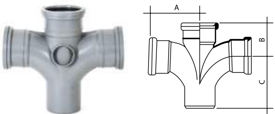
Cross Tee 87.5°
