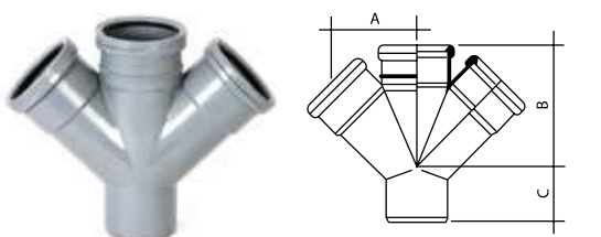
Double Branch 45°
