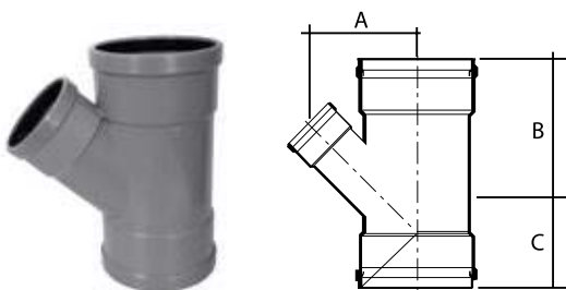
Y Branch 45° (Reducing)
