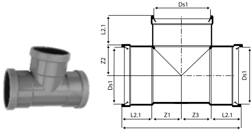
Tee 88° (3 Socket)
