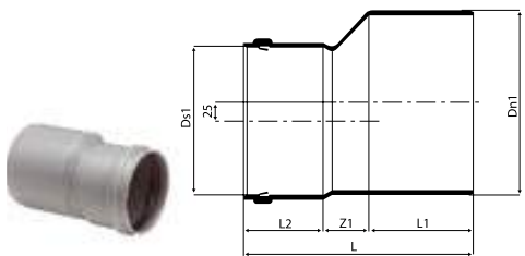
Eccentric Reducer (Sockets / Spigot) Long
