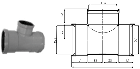
Reducing Tee 88° (3 Socket)
